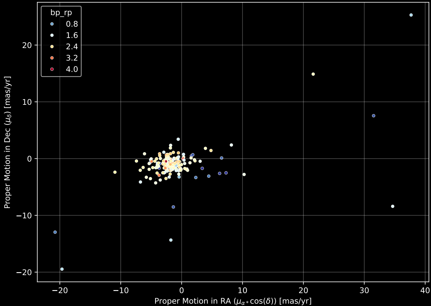
APOGEE DR17 Field: [116-04] Proper Motion Diagram (n= 173)
