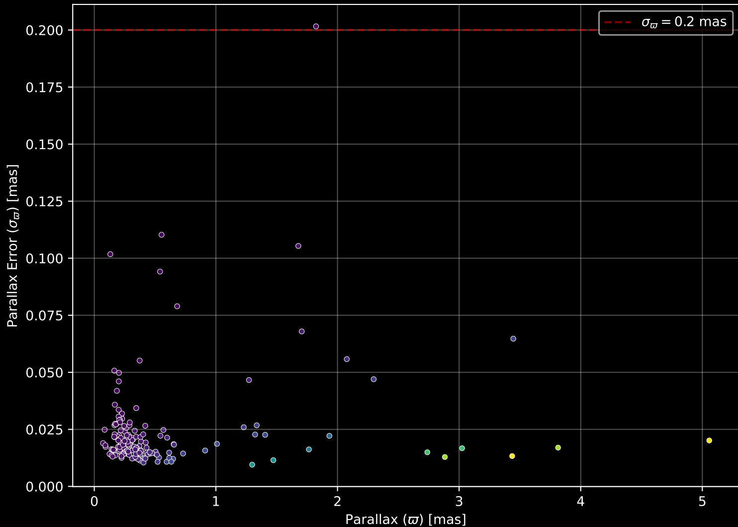
APOGEE DR17 Field: [116-04] Parallax Quality (n= 173)
