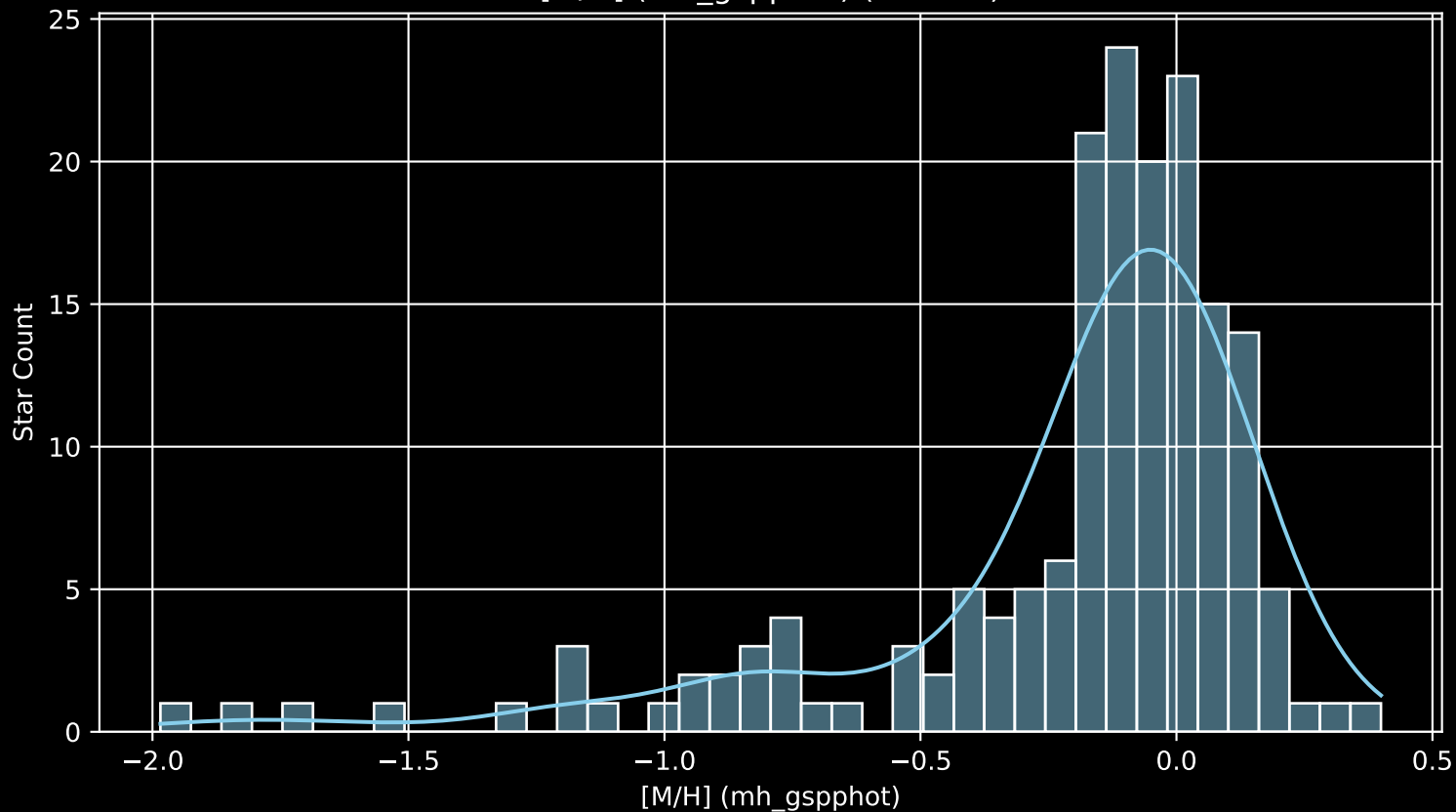
APOGEE DR17 Field: [116-04 [M/H] (mh_gspphot) (n= 173)
