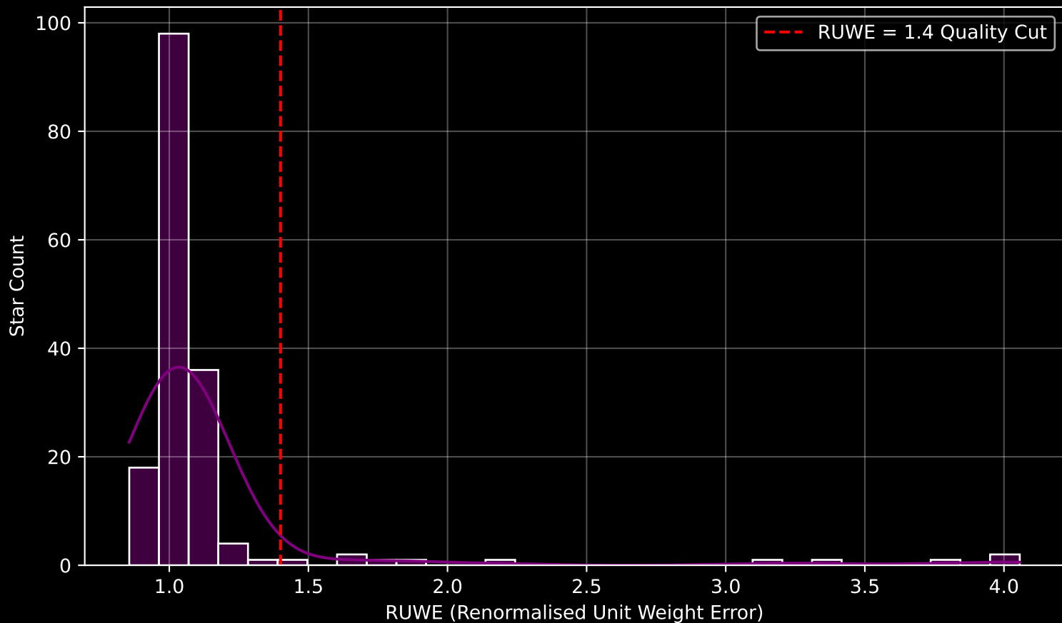
GAPOGEE DR17 Field [116-04] RUWE Distribution (n= 168)
