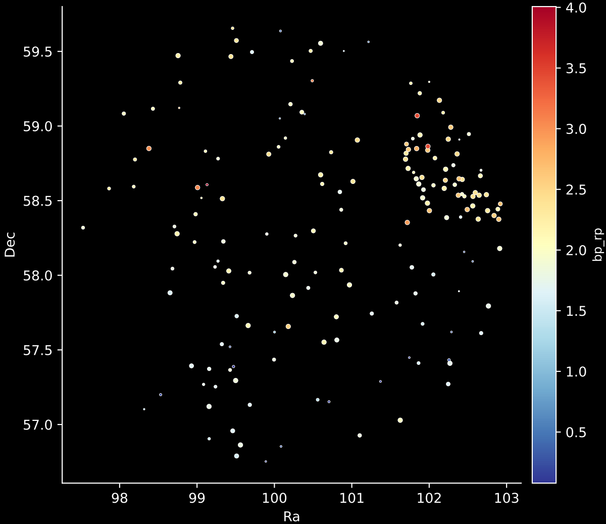
APOGEE DR17 Field: [116-04] Stars: 173
